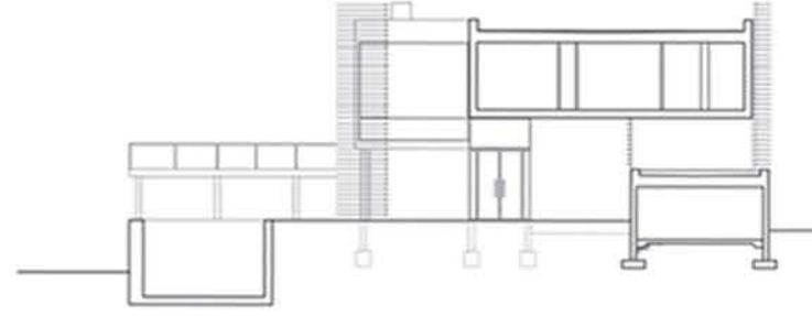
剖图B Section B
